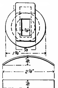
THE SCHROYER-THOMPSON PISTON-TRAVEL INDICATOR.
